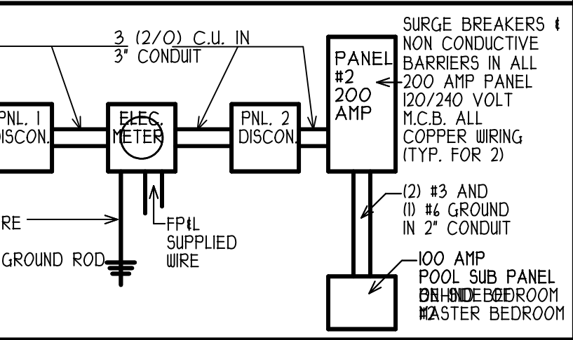
400 AMP ELEC. RISER DIAGRAM
